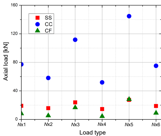
Fig. 4. Variation in buckling loads for the three boundary conditions under various VALs.
