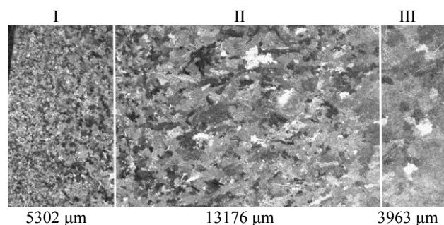
Fig. 4. Image of the macrostructure of the cut fragment of the sleeve with marked areas. Stage 2: CuSi3Zn3FeMn, 1500 rpm
