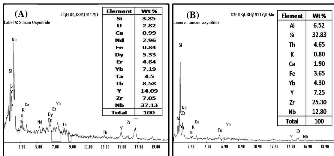
Fig. 10. EDX analysis data of float (A), sink (B) products
