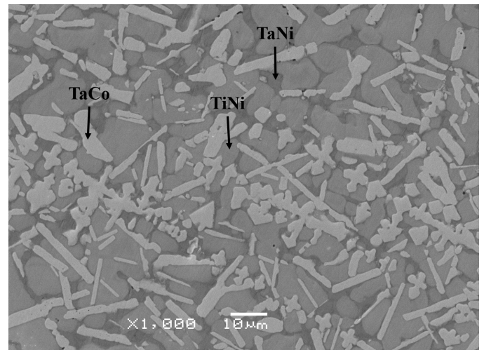
Fig. 3. SEM microstructure images with assigned phases for studied alloy
