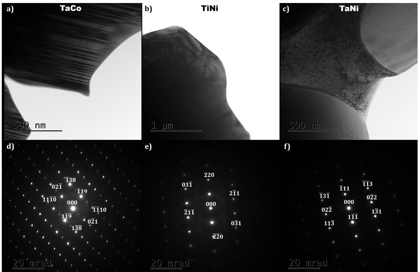
Fig. 5. Bright field and SAED images for (a-d) TaCo, (b-e) TiNi and (c-f) TaNi phases
