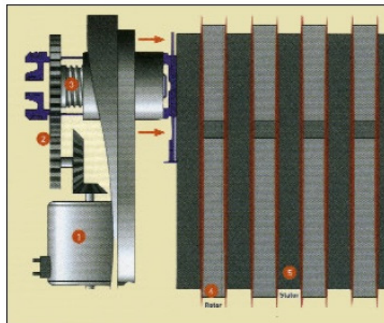
Fig. 4. Modern electric drive used in aviation brake for Boeing 787 Dreamliner. (source: Internet)
