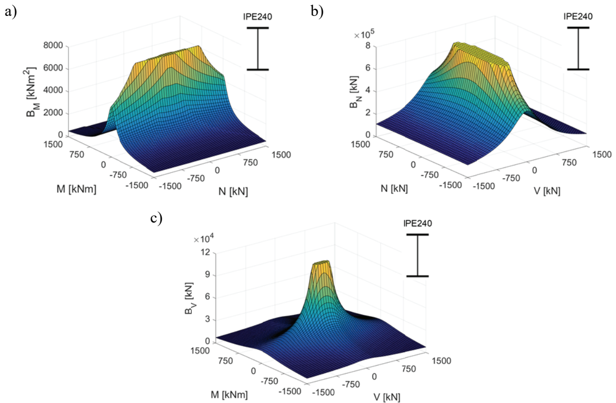
Fig. 3. Bending, tensile and shear stiffnesses, B_M , B_N and B_V , for the IPE240 depending respectively on: a) bending moment and normal force ( V = 0 ), b) normal force and shear force ( M = 0 ), and c) bending moment and shear force ( N = 0 )
