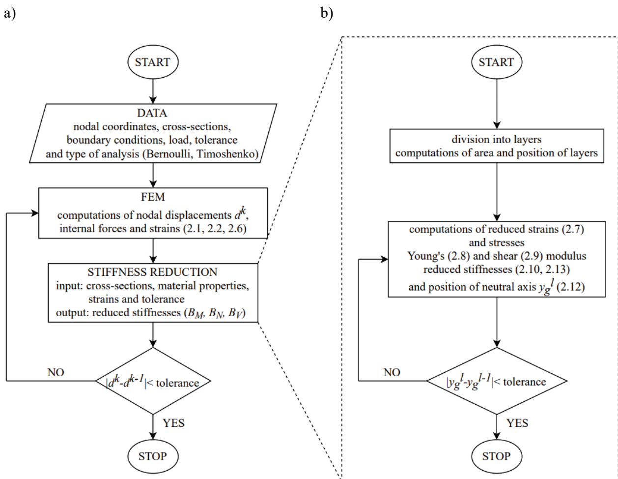
Fig. 1. Block diagrams of the computational algorithm of the proposed method: a) the overall finite element method framework ( k is the finite element method iteration number), and b) detailed framework of stiffness reduction function ( l is the iteration number of deriving neutral axis position)
