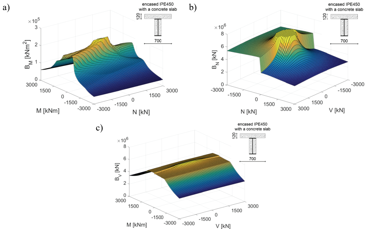
Fig. 5. Bending, tensile and shear stiffnesses, B_M , B_N and B_V , for the encased IPE450 with a concrete slab depending respectively on: a) bending moment and normal force ( V = 0 ), b) normal force and shear force ( M = 0 ), and c) bending moment and shear force ( N = 0 )
