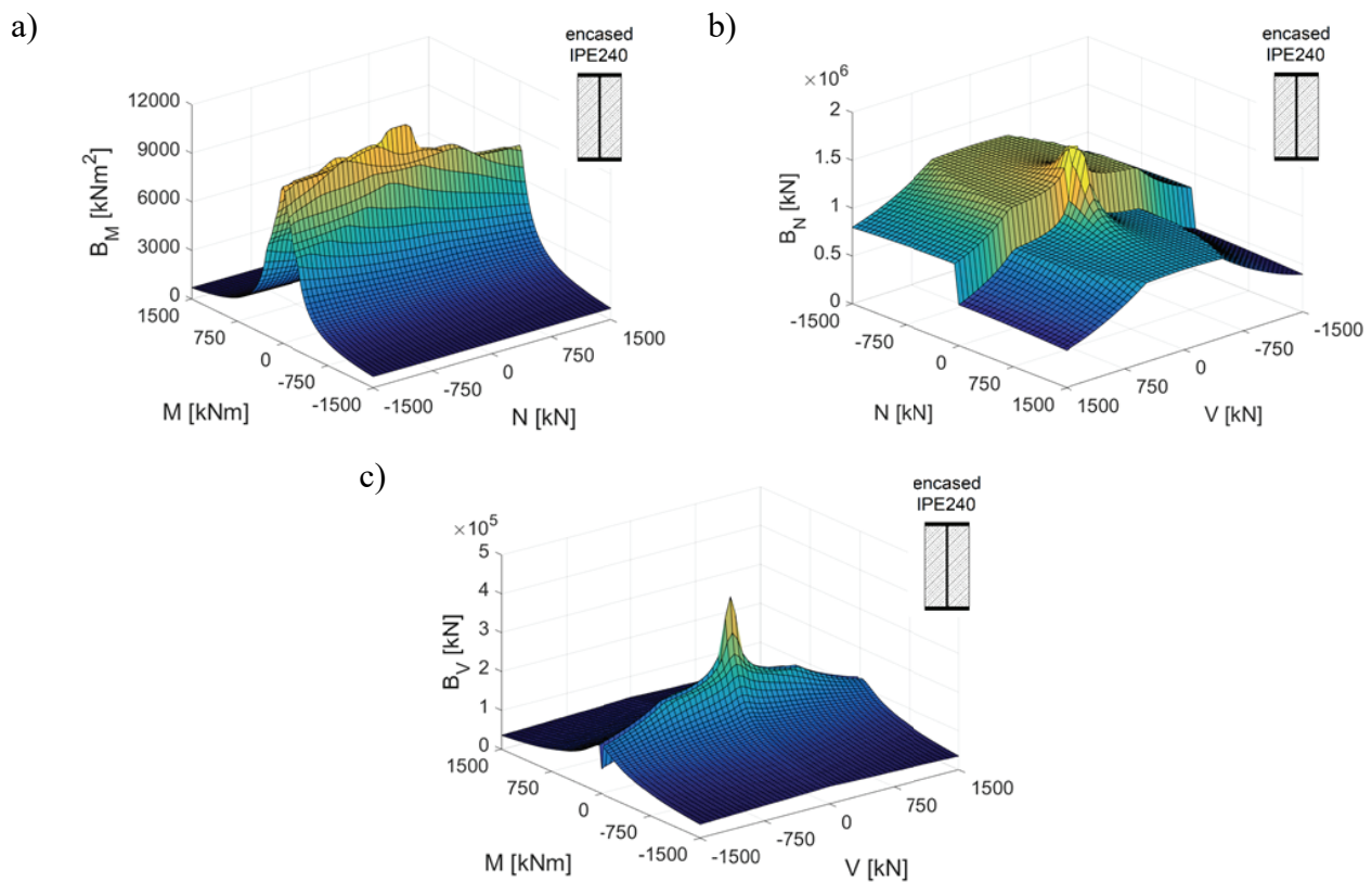
Fig. 4. Bending, tensile and shear stiffnesses, B_M , B_N and B_V , for the encased IPE240 depending respectively on: a) bending moment and normal force ( V = 0 ), b) normal force and shear force ( M = 0 ), and c) bending moment and shear force ( N = 0 )
