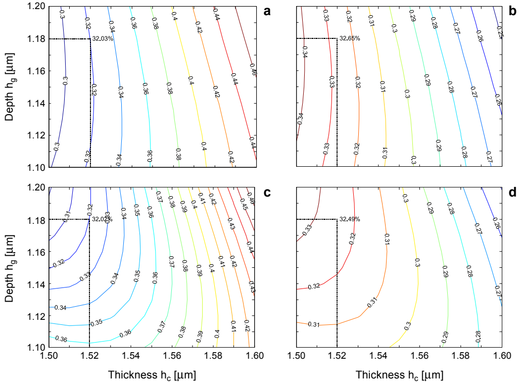
Fig. 2. Diffraction efficiency versus grating depth and thickness of the connecting layer with the duty cycle of 0.5 and period of 1910 nm for the wavelength of 1550 nm: TE polarization diffracted into the 0th order (a), TE polarization diffracted into the 1st order (b), TM polarization diffracted into the 0th order (c), and TM polarization diffracted into the 1st order (d).
