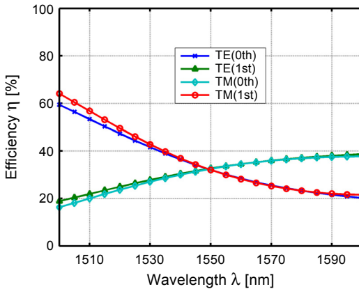
Fig. 4. Diffraction efficiency versus incident wavelength with the usual duty cycle of 0.5 for the optimized grating depth and connecting layer thickness h_g = 1.18 \mu\text{m} and h_c = 1.52 \mu\text{m} under the normal incidence.
