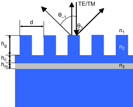
Fig. 1. Schematic of a highly-efficient three-port output by metal-mirror-based grating.
