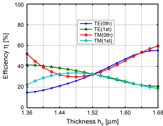
Fig. 3. Diffraction efficiency versus thickness of the connecting layer with the duty cycle of 0.5, the period of 1910 nm and the depth of 1.18 \mu\text{m} for the wavelength of 1550 nm.
