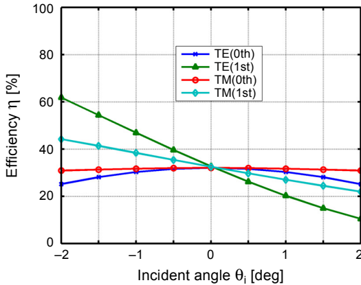
Fig. 5. Diffraction efficiency versus angle of incidence for the wavelength of 1550 nm with the optimized grating profile parameters.
