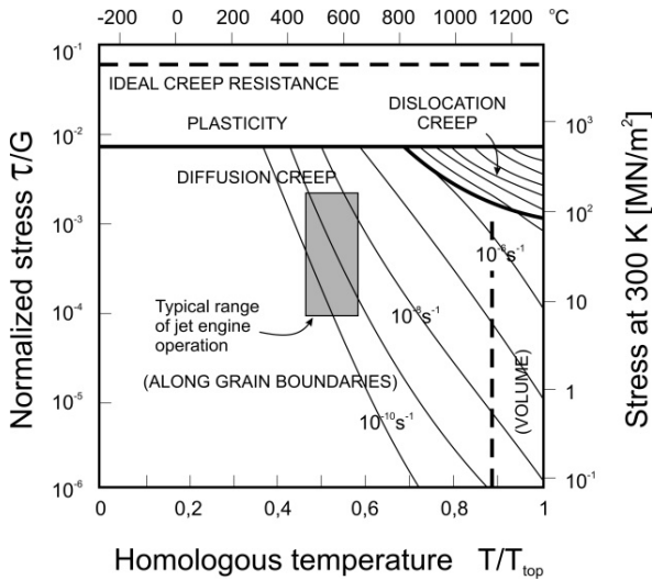
Fig. 1. Map of deformation mechanisms in MAR-M-200 alloy, grain size 100 μm [8]
