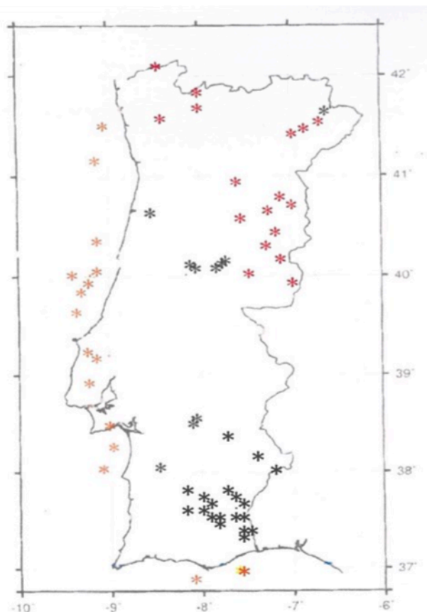
Fig. 1. Location of points with heat flow density values. Measurements were done in boreholes (dark), oil/gas wells (brown) and using numerical models (red).
