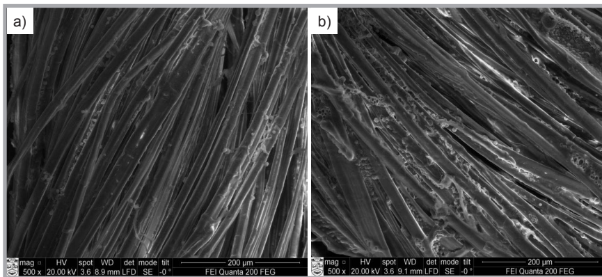
Figure 8. SEM micrographs (500 x magnification) of ramie fibre of treated terry fabric with weft density of 16 cm -1 and different binder concentrations: a) 20 g/dm 3 , b) 95 g/dm 3 .
