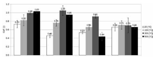
Fig. 4. Mean values of the friction coefficient obtained during the tests
