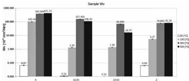
Fig. 5. Values of the wear rate after tests in applied temperatures separately for all tested sample materials (logarithmic scale)
