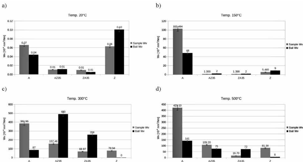
Fig. 3. Wear rate of the sample and countersample tested at temperatures: a) 20°C, b) 150°C, c) 300°C, d) 500°C
