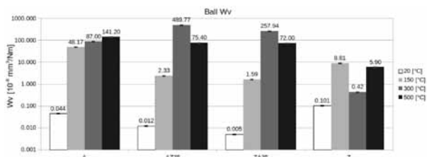
Fig. 6. Wear rate values of countersamples after tests in applied temperatures separately for all tested sample materials (logarithmic scale)
