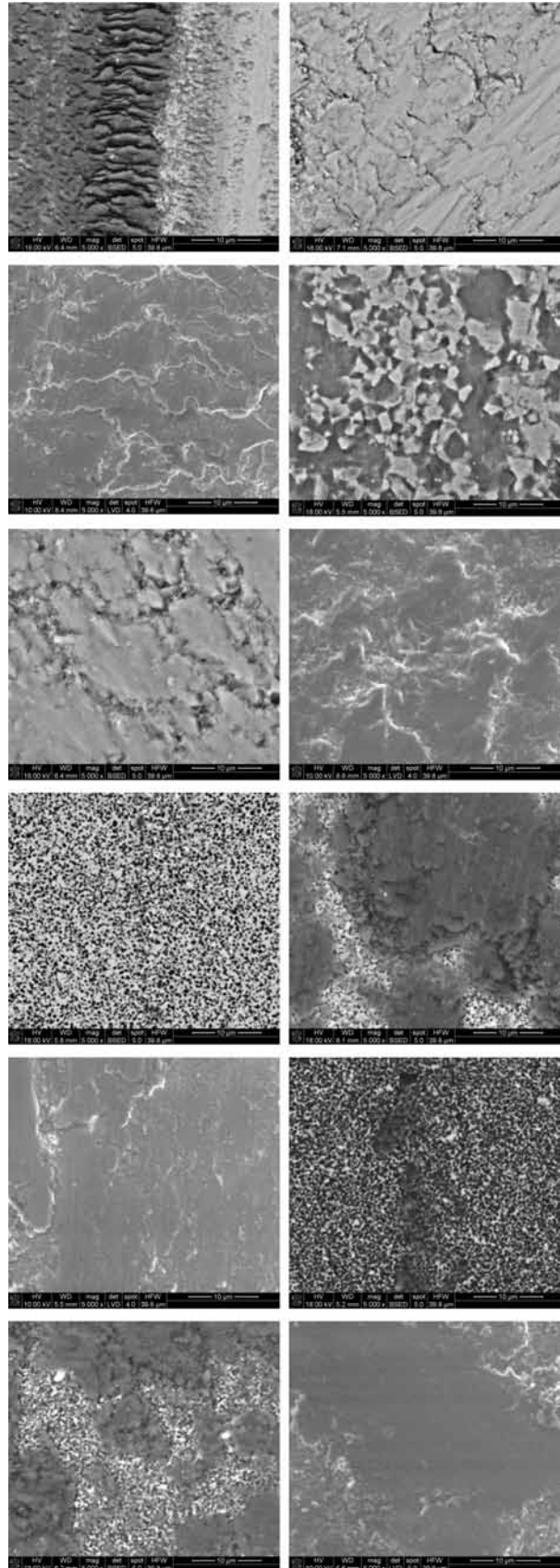
Fig. 7. SEM images of wear tracks: in the sequence from the left top Z, A, AZ35, and ZA35; in rows from the left for 20, 300, and 500°C
