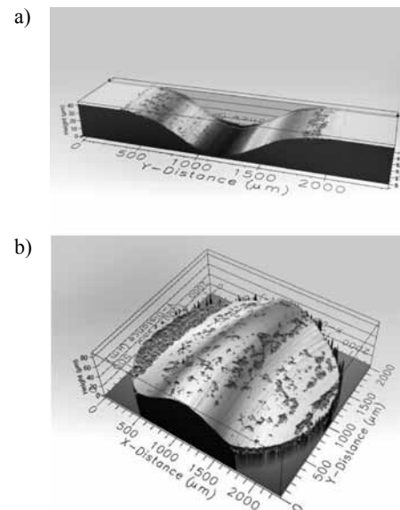
Fig. 2. The surface profiles of: a) sample b) ball
