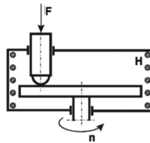
Fig. 1. Scheme of the friction pair in T-21 tribometer
