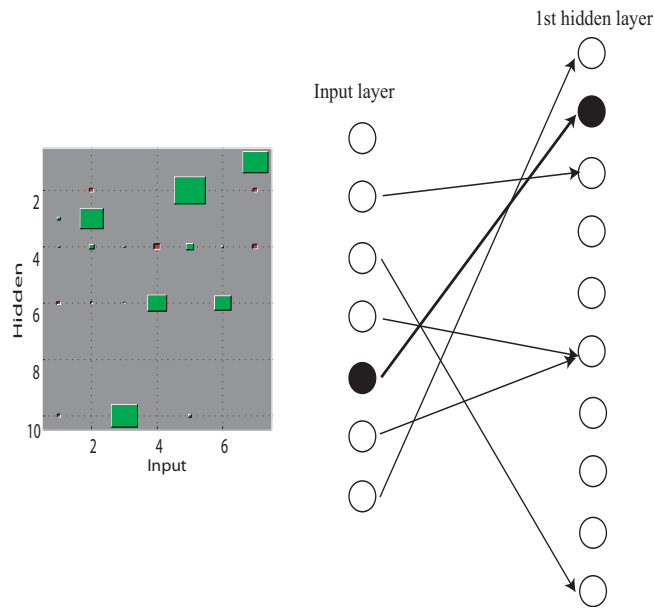
Figure 11. Connection weights in Hinton diagram (a) and the conventional diagram (b), corresponding to those in Figure 10(a4) for the wholesale data set.
