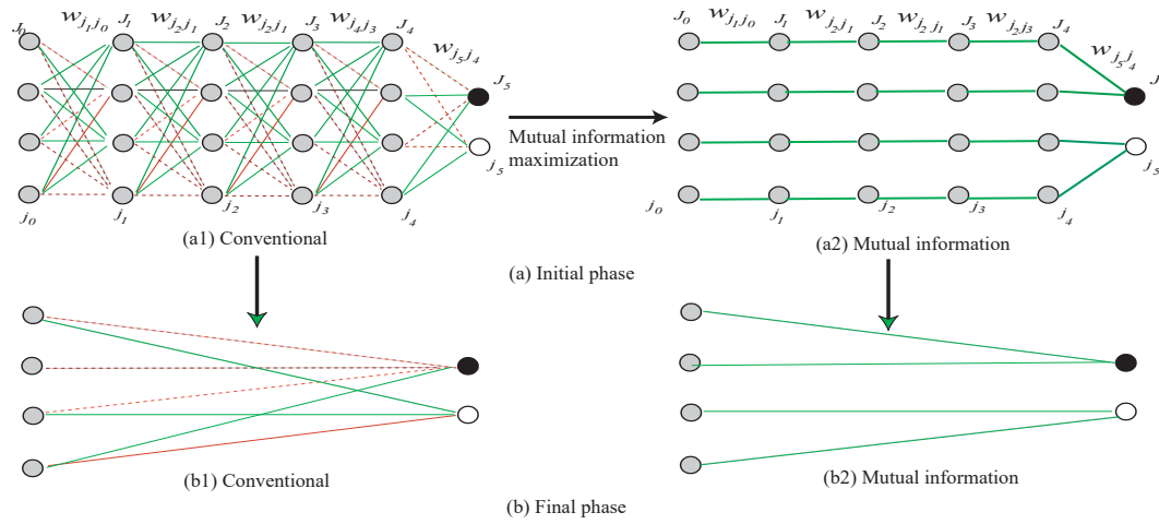
Figure 3. Collective weights
