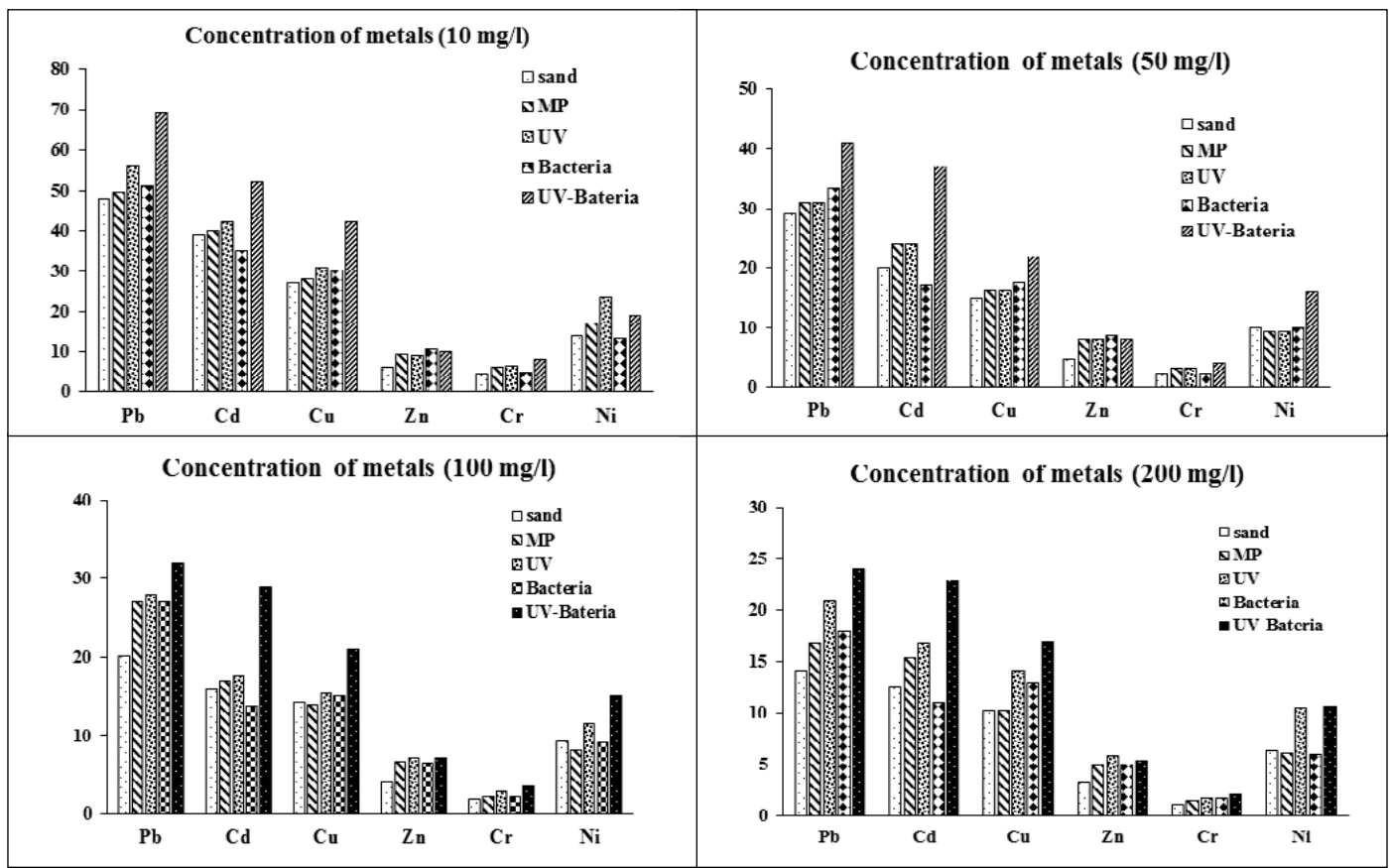
Fig. 4. Percentage of adsorption of heavy metals on various compounds of sand and micro-plastics, under UV irradiation and bacterial culture at concentrations of 10, 50, 100 and 200 mg/l
