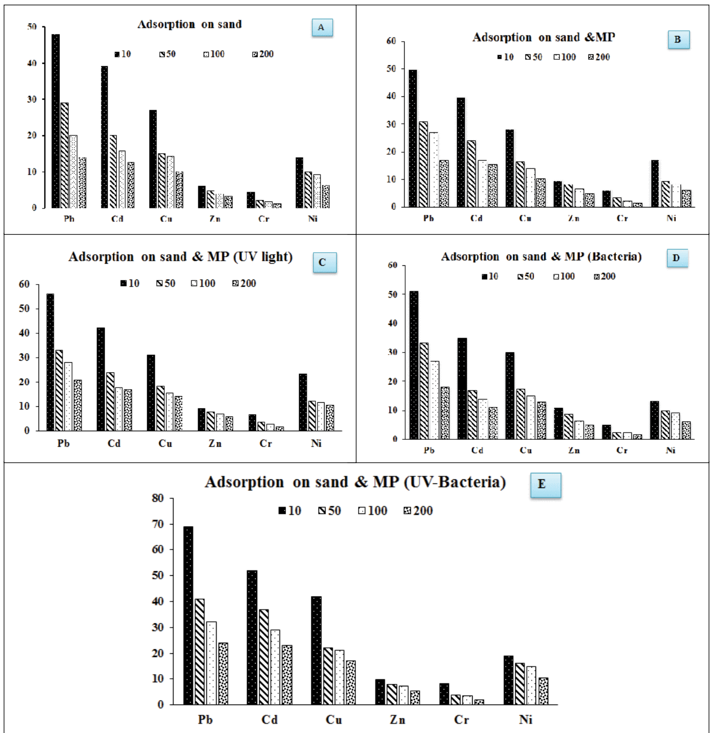
Fig. 3. Adsorption of heavy metals on A) Sand, B) Sand and micro-plastics C) Sand and micro-plastics exposed to UV D) Sand and micro-plastics containing bacteria E) Sand and micro-plastics containing bacteria exposed to UV
