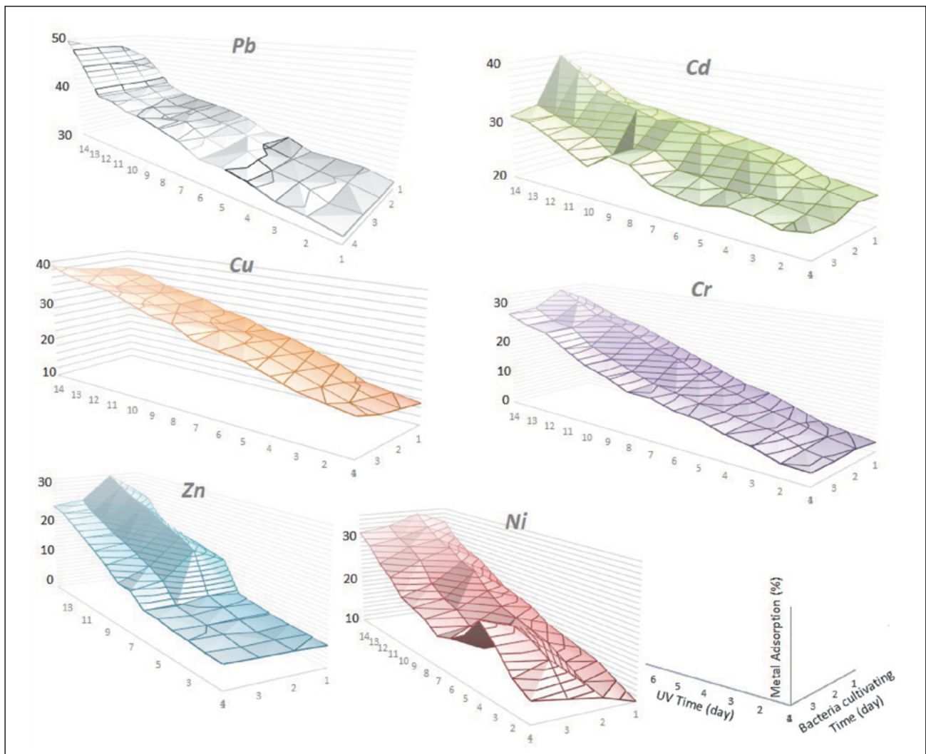
Fig. 1. Results of heavy metal adsorption during bacterial culture for 1 to 4 days and UV exposure time from 1 to 14 days
