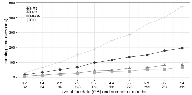
Fig. 2. Experiments with Siemens data over 32–319 months.
