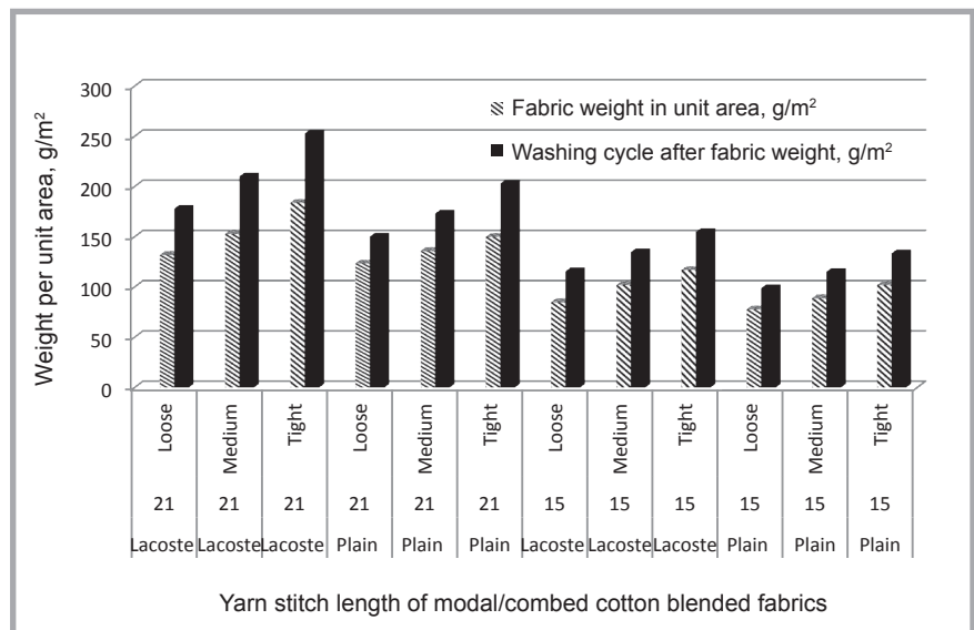
Figure 1. Effect of weight per unit area of modal/combed cotton blended fabrics.
