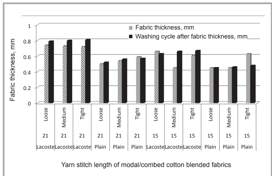
Figure 2. Effect of fabric thickness of modal/combed cotton blended fabrics.
