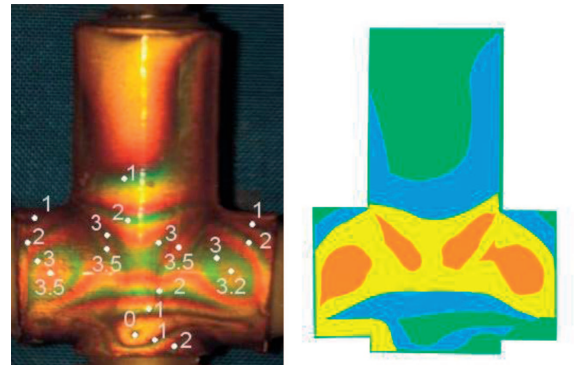
Fig. 16. Stress distribution: working load = 4,0 Nm, steel washer, compressing
