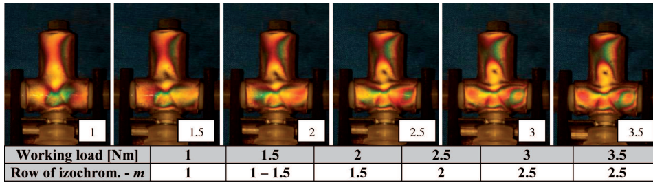
Fig. 7. Isochromatics under the working load from M=1 to 3,5 Nm – connection stretched (force acting downward), steel washer
