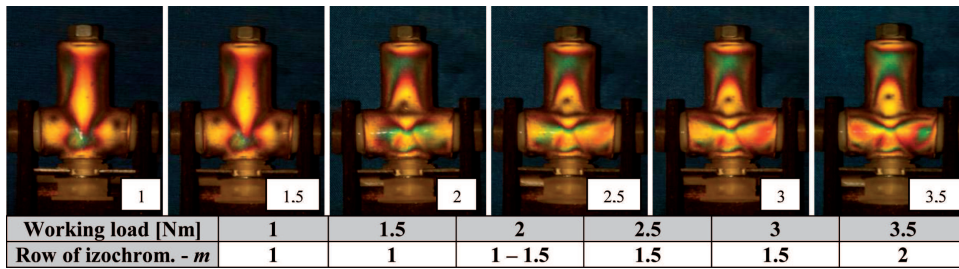
Fig. 8. Isochromatics under the working load from M=1 to 3,5 Nm – connection stretched (force acting downward), FullCure 720 washer
