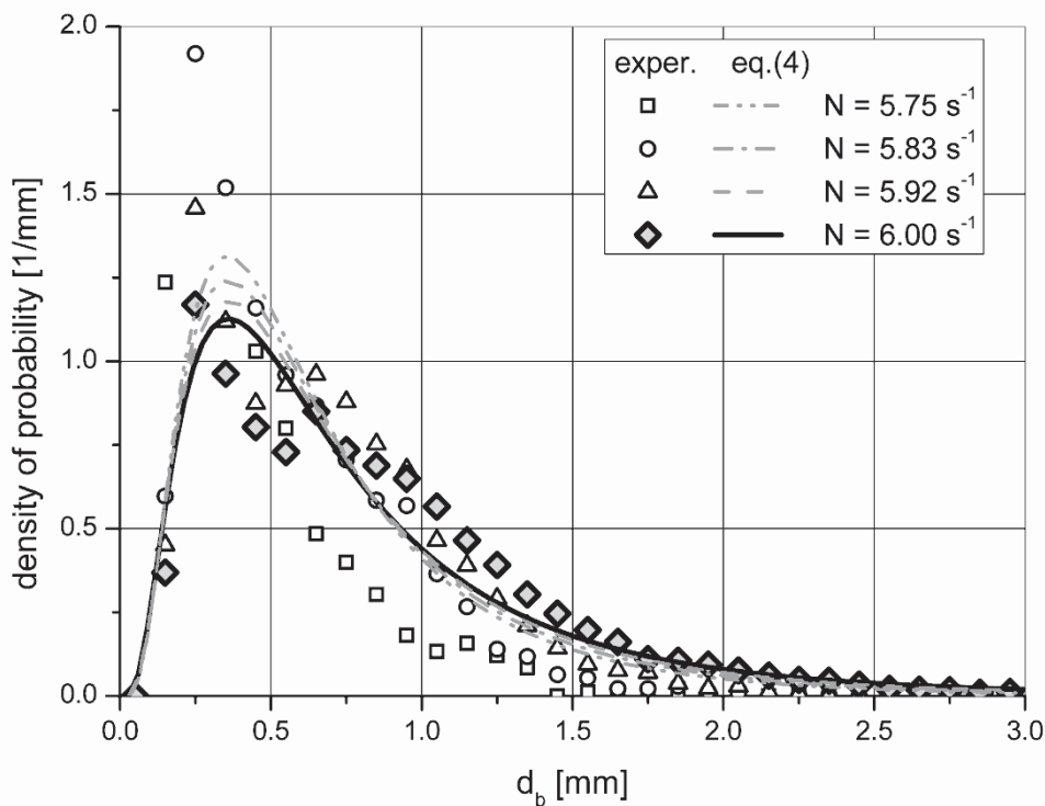
Fig. 3. Bubble diameter distribution (Stelmach, 2007)
