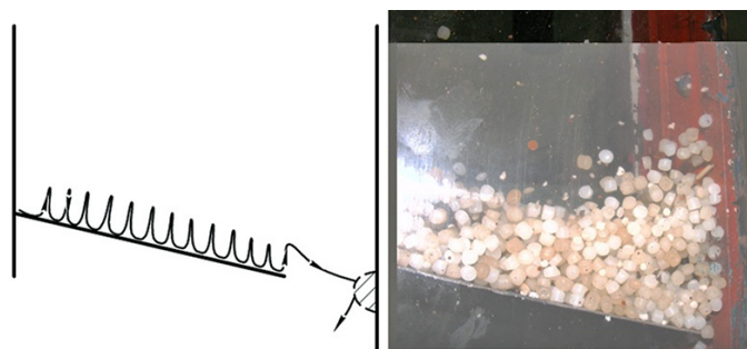
Fig. 5. Dryer's operation in the weighted layer mode of the dispersed material
