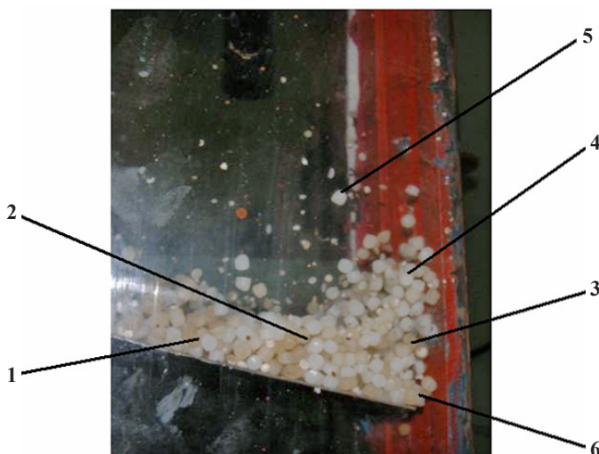
Fig. 6. Distinctive zones of dispersed material motion in the gravitational shelf device: 1 – weighted layer creation zone on the shelf; 2 – zone of lowering the weighted layer intensity; 3 – vortex creation zone; 4 – zone of increased velocity of the dispersed material motion over the outloading gap; 5 – separation zone of finely dispersed material; 6 – outloading zone of the dispersed material from the shelf
