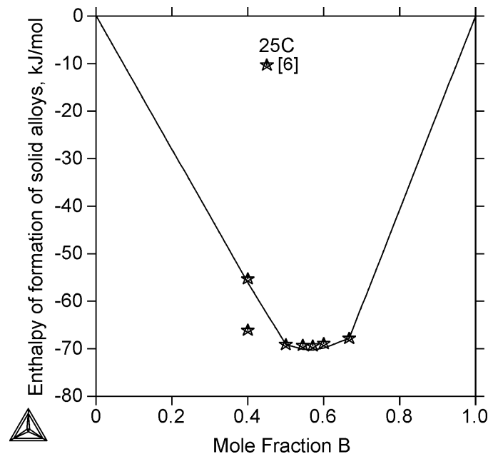
Fig. 5. Calculated enthalpy of formation of solid B-V alloys at 25°C, together with experimental data points [6]. Calculations of are practically identical to those of [6]. The reference states used are pure bcc V and pure beta-rhombo B
