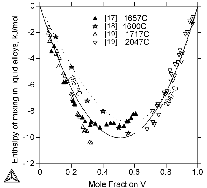
Fig. 4. Calculated enthalpy of mixing of liquid Fe-V alloys at 2047°C and 1657°C, together with experimental data points [17-19]. Solid lines refer to the current calculations and dotted lines refer to those of [7]. The reference states used are pure liquid Fe and V
