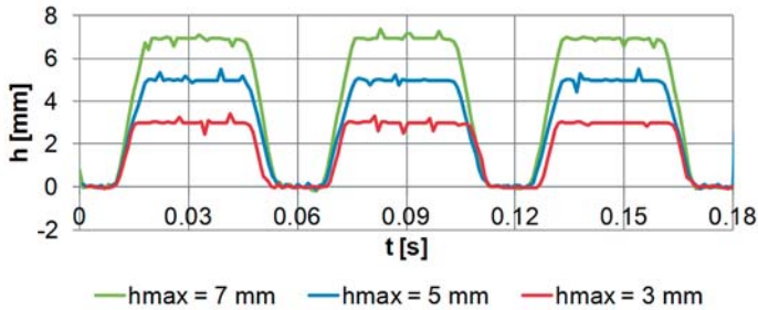
Fig. 4. Measured values of the valve lift h against time t ; loading frequency f = 16 Hz, valve stroke h_{max} = 7 mm, h_{max} = 5 mm, and h_{max} = 3 mm, respectively
