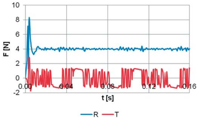
Fig. 10. Values of friction force T and of normal force R against time t , obtained during simulations; loading frequency f=16 Hz, valve stroke h_{max}=5 mm
