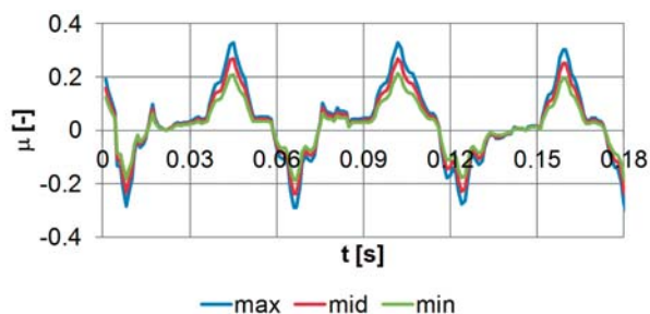
Fig. 8. Calculated values of friction coefficient \mu between valve and its guide against time t ; loading frequency f = 16 Hz, valve stroke h_{max} = 5 mm
