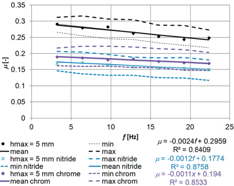
Fig. 9. Calculated values of friction coefficient \mu between valve and its guide against loading frequency f ; valve stroke h_{max} = 5 mm, valve uncoated, nitrided, coated by chromium layer
