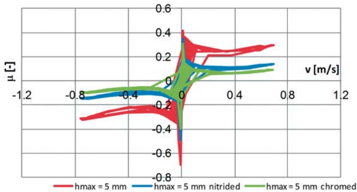
Fig. 12. Values of friction coefficient \mu against sliding velocity v ; loading frequency f = 16 Hz, valve stroke h_{max} = 5 mm, without protective layer, nitrided and chromed
