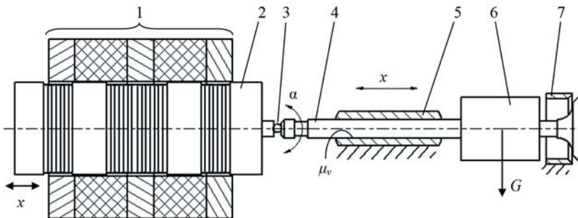
Fig. 3. The model of the assembly consisted of movable coil the drive and valve bearing in its guide and loaded by additional weight; 1 - immovable part of the drive, 2 - movable coil, 3 - spherical joint, 4 - valve, 5 - guide, 6 - additional weight, 7 - seat insert
