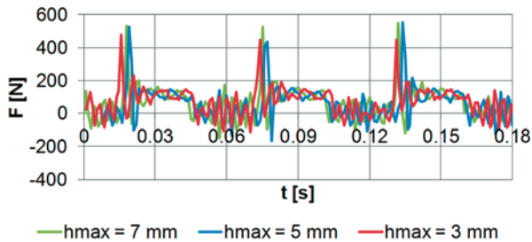
Fig. 6. Measured values of the impact force F between valve and its seat insert against time t ; loading frequency f = 16 Hz, valve stroke h_{max} = 7 mm, h_{max} = 5 mm and h_{max} = 3 mm, respectively
