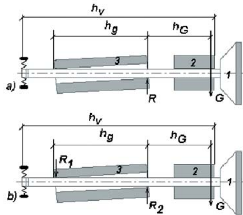
Fig. 2. The scheme of loading for the valve - added mass - guide assembly; 1 - valve, 2 - added mass, 3 - guide; a) loading case, when reaction R between valve stem and its guide has existed in only one place, b) loading case, when reactions R1 and R2 between valve stem and its guide have existed in two places
