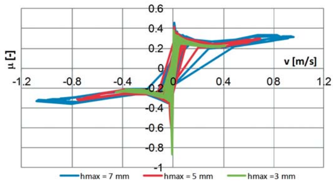
Fig. 11. Values of friction coefficient \mu against sliding velocity v ; loading frequency f=16 Hz, valve stroke, h_{max}=7 mm, h_{max}=5 mm and h_{max}=3 mm
