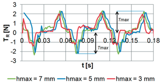
Fig. 7. Measured values of the friction force T_R between valve and its guide against time t ; loading frequency f = 16 Hz, valve stroke h_{max} = 7 mm, h_{max} = 5 mm and h_{max} = 3 mm, respectively, T_{max} - maximum friction force during valve displacement against its guide
