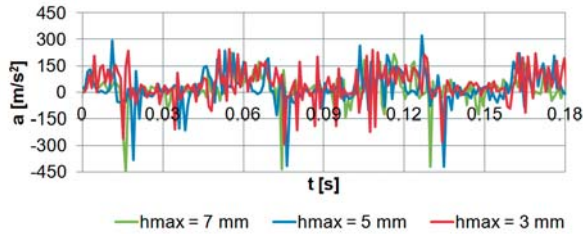
Fig. 5. Measured values of the valve acceleration a against time t ; loading frequency f = 16 Hz, valve stroke h_{max} = 7 mm, h_{max} = 5 mm and h_{max} = 3 mm, respectively
