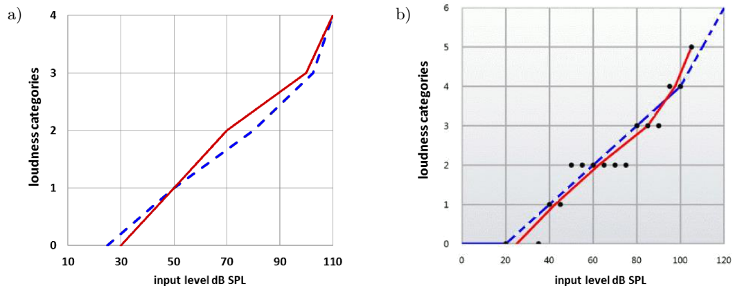
Fig. 7. Examples of loudness scaling results: 1000 Hz, normal hearing, a) obtained in the developed test – vertical scale as in Fig. 6; b) obtained in the LGOB test – vertical scale as denoted in Fig. 2; the dashed line refers to the LGOB reference function.
