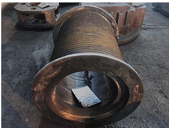
Fig. 1. Rope drum cast
