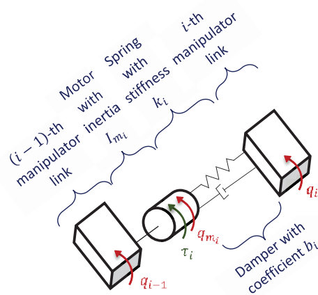
Figure 2. Schematic view of flexible joint with viscous damping
