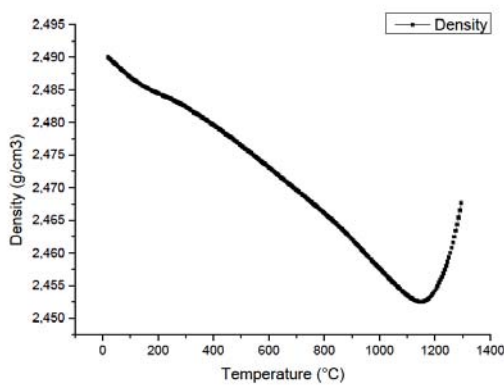
c) Density of shell measured at different temperatures
