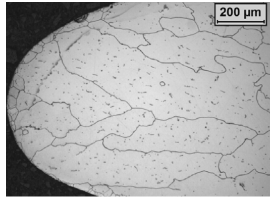
d) Grain structure in leading edge of blade at cast temperature 1560 °C with 11 mm shell
