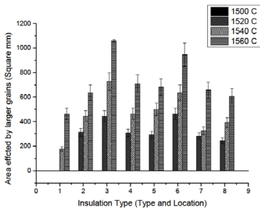
c) Effect of insulation type on size of porosity at different temperatures
