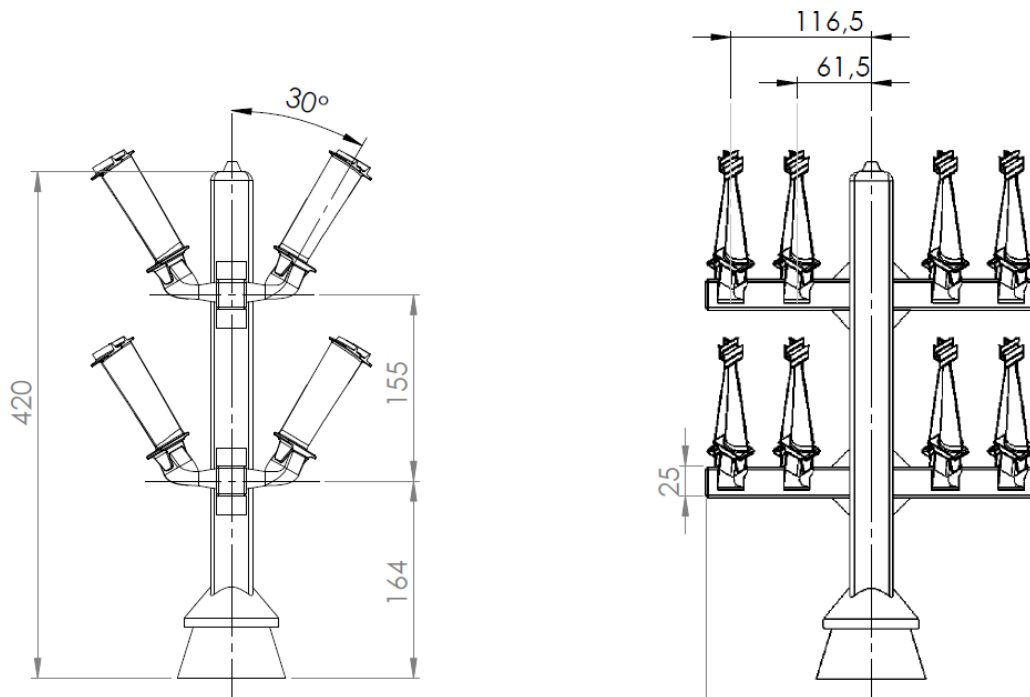
Fig. 2. Tree design for blade casting, all dimensions in millimetres
