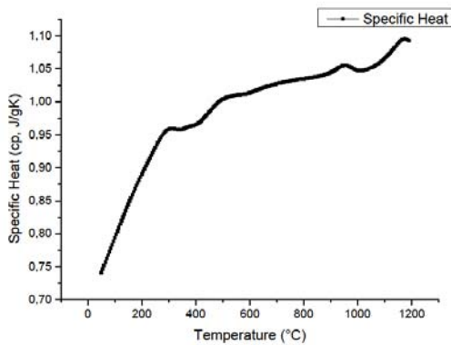
a) Specific heat of shell measured at different temperatures
