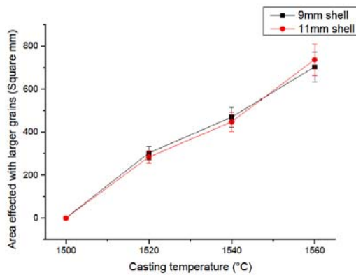
a) Effect of casting temperature on Porosity at two different shell thickness
