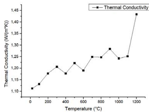
d) Thermal conductivity of shell measured at different temperatures
