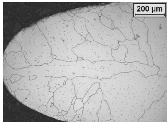
b) Grain size at leading edge of the blade cast with 11 mm shell cast at 1560 °C
