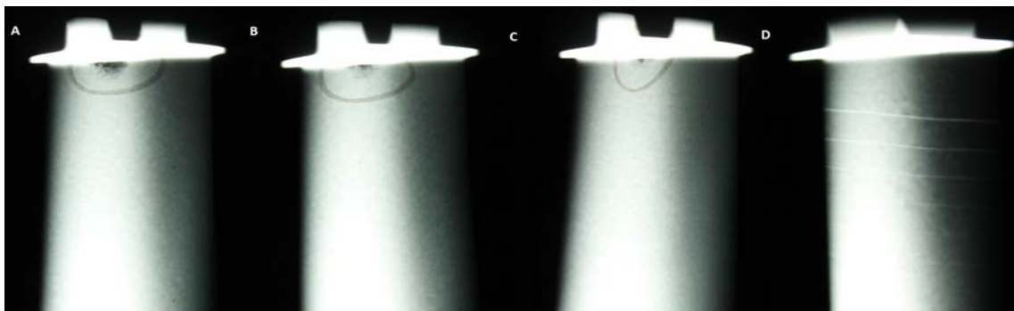
Fig. 6. Indication of porosity at different cast temperatures A) 1500 °C, B) 1520 °C, C) 1540 °C, D) 1560 °C
