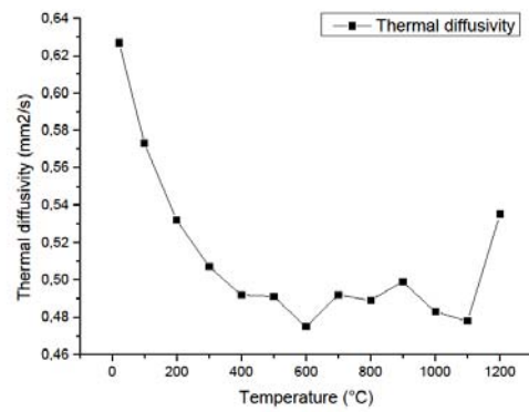
b) Thermal diffusivity of shell measured at different temperatures
