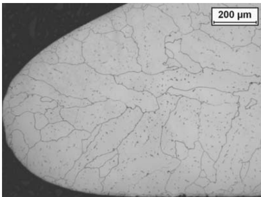
a) Grain size at leading edge of the blade cast with 9 mm shell cast at 1560 °C
