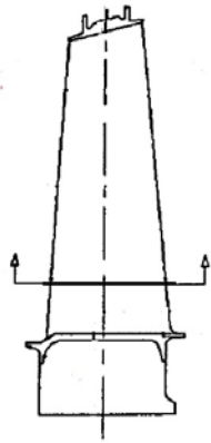
Fig. 4. Sample location for micro structure evaluation.
