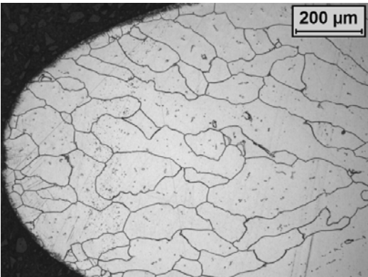
c) Grain structure in leading edge of blade at cast temperature 1520 °C with 11 mm shell
