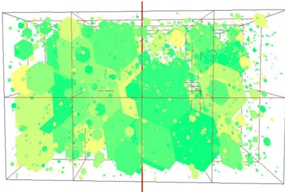
Fig. 12. Number 1, the initial number is 3, the initial length is 120, trend is 45°, tendency is 30°, hexagon
