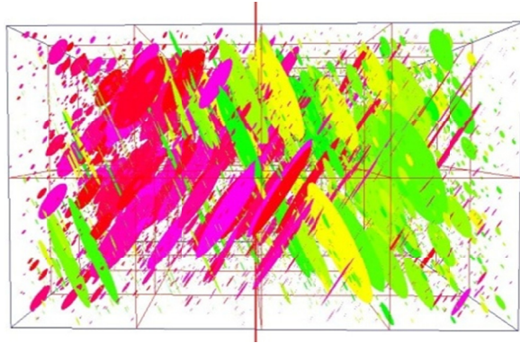
Fig. 11. Number 2, the initial number is 3, the initial length is 120, trend is 45°, tendency is 30°, disc
