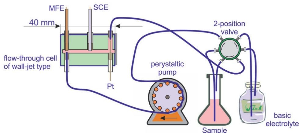
Fig. 1. A three-electrode measuring cell, consisting of a mercury film working electrode (MFE) based on glassy carbon, a saturated calomel reference electrode (SCE) and a platinum wire auxiliary electrode
