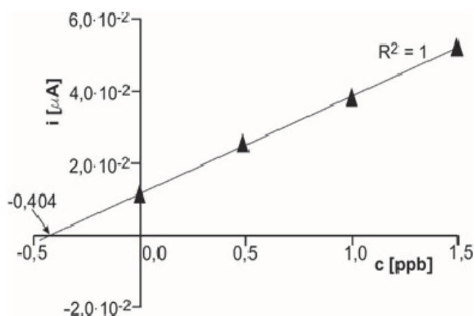
Fig. 3. Standard addition curve for determination of thallium concentration with 3 additions
