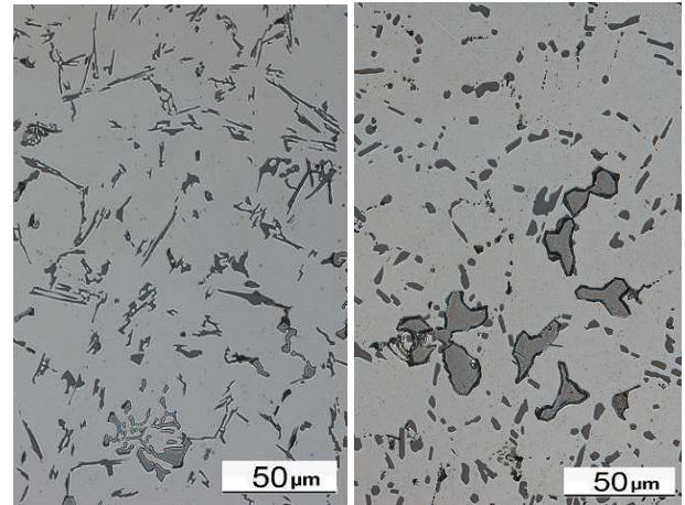
a) Cast state b) after heat treatment
