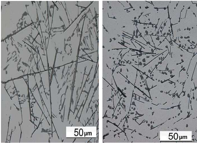
a) Cast state b) after heat treatment
