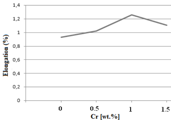
Fig. 8. Ductility of alloys after chrome addition
