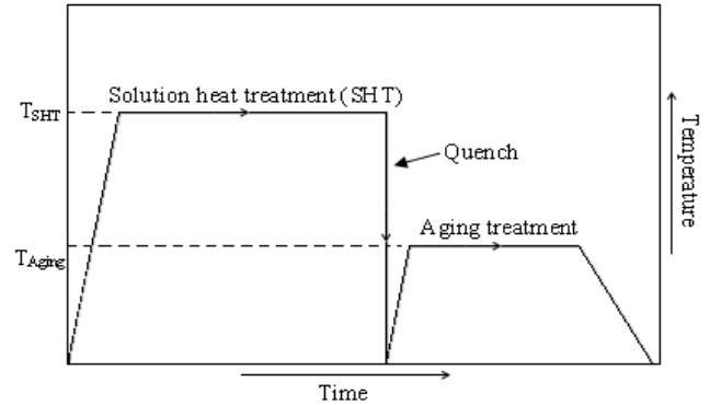
Fig. 1. Heat treatment of alloy
