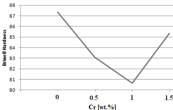
Fig. 9. Brinell Hardness of alloys after chrome addition
