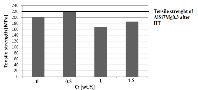
Fig. 7. Tensile strength of alloys after chrome addition and heat treatment
