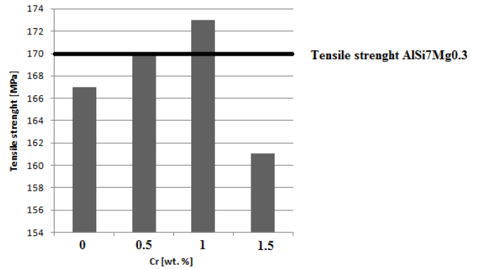
Fig. 6. Tensile strength of alloys after chrome addition
