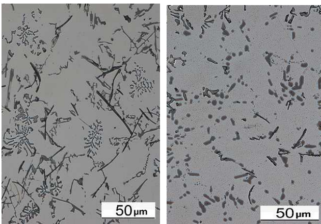
a) Cast state b) after heat treatment
