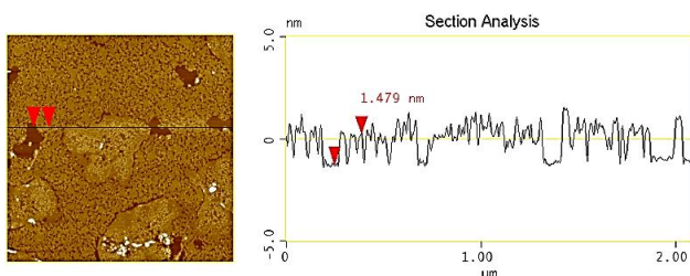
Fig. 3. Section analysis of DA skeletonized layer.
