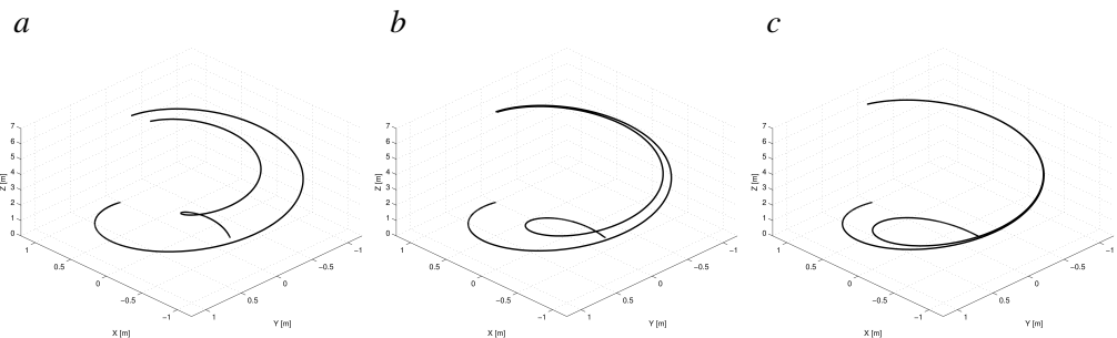
Figure 5: Trajectory of manipulator for linear time parametrization: a – trajectory for K_p = 0.02 , b – trajectory for K_p = 0.05 , c – trajectory for K_p = 0.1
