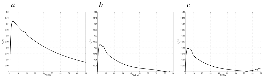
Figure 12: Curvilinear error e_s = s - s_d for quadratic time parametrization: a – error e_s for K_p = 0.02 , b – error e_s for K_p = 0.05 , c – error e_s for K_p = 0.1
