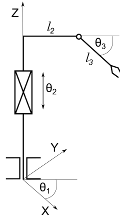
Figure 4: Manipulator RTR – object of simulation
