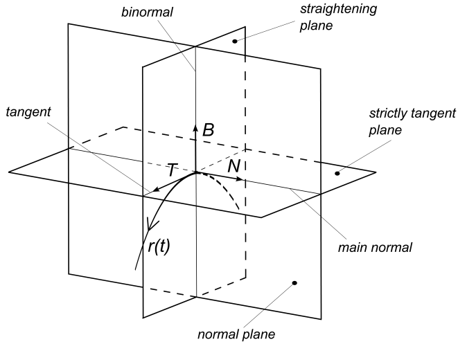
Figure 2: Frenet trihedron.
