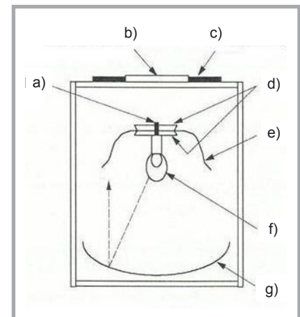
Figure 1. Typical Cusick drape meter; a) specimen fixing needle, b) central disc lid, c) paper ring, d) specimen support discs, e) fabric specimen, f) spot light, g) parabolic mirror.
