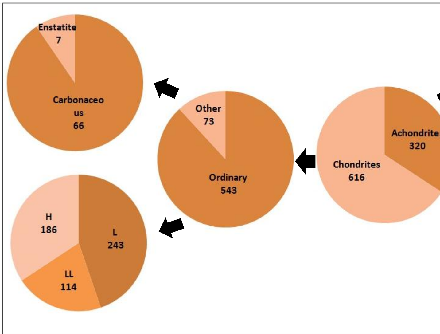
Fig. 4. Moroccan meteorite finds Statistic.
