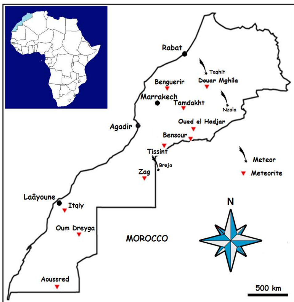
Fig. 1. Map showing the distribution of meteorite falls from Morocco.
