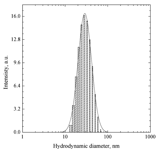
Fig. 1. The size distribution of AuNPs synthesized by reduction of gold(III) complex ions using sodium citrate. Conditions: C_{0,Au(III)} = 0.25 mM, C_{NaCit} = 1.25 mM, Temperature ca. 100°C
