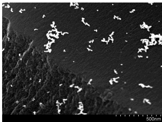
Fig. 7. SEM micrographs of AuNPs deposited on the 10-CO Organosorb AC modified with triethylenetetramine molecules. Conditions: C_{0,Au(III)} = 0.25 mM, C_{NaCitrate} = 1.25 mM, Temperature ca. 100^{\circ}\text{C}
