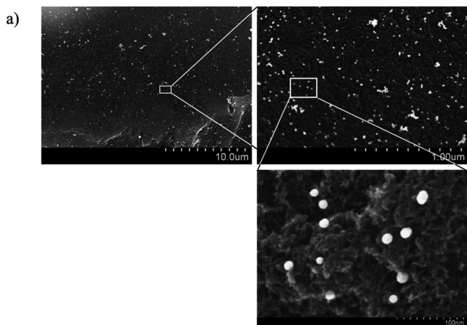
Fig. 7. SEM micrographs of AuNPs deposited on the 10-CO Organosorb AC modified with triethylenetetramine molecules. Conditions: C_{0,Au(III)} = 0.25 mM, C_{NaCitrate} = 1.25 mM, Temperature ca. 100^{\circ}\text{C}
