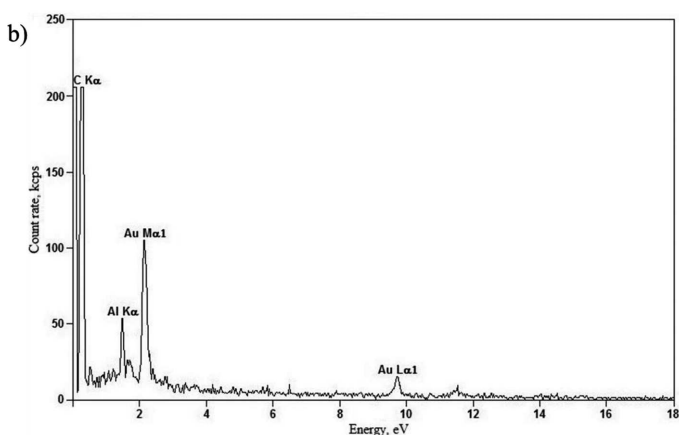
Fig. 5. a) SEM micrographs of AuNPs deposited on 10-CO Organosorb AC modified with ethanolamine molecules; b) EDS analysis of deposits. Conditions: C_{0,Au(III)} = 0.25 mM, C_{NaCitrate} = 1.25 mM, Temperature ca. 100^{\circ}\text{C}
