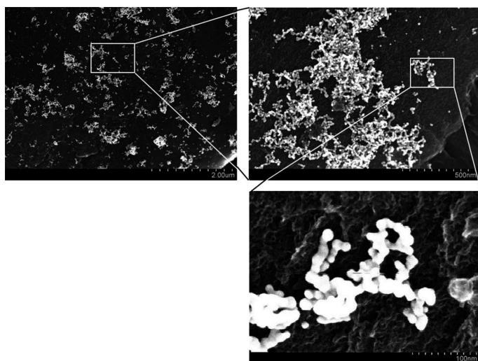
Fig. 6. SEM micrographs of AuNPs deposited on the 10-CO Organosorb AC modified with diethylenetriamine molecules. Conditions: C_{0,Au(III)} = 0.25 mM, C_{NaCitrate} = 1.25 mM, Temperature ca. 100^{\circ}\text{C}
