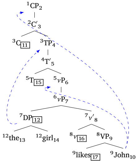
Figure 7: Modified recursive descent operates correctly over MG derivation trees
