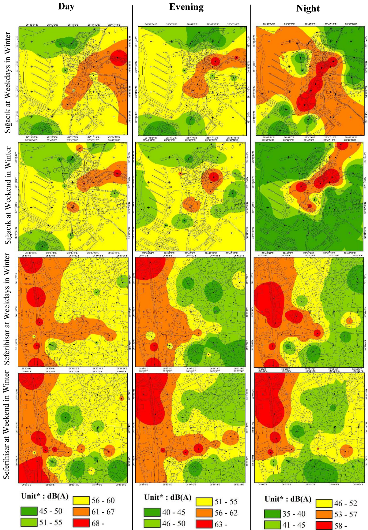
Fig. 4. Daytime, evening and night noise maps of study area in winter period (* the scales based on the noise limit values in Turkey).
