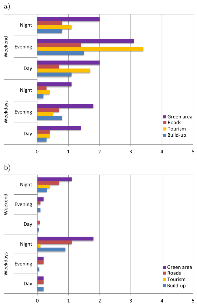
Fig. 7. The land (area [ha]) uses in which the noise exceeded the limit values in Sığacık: a) in summer, b) in winter.
