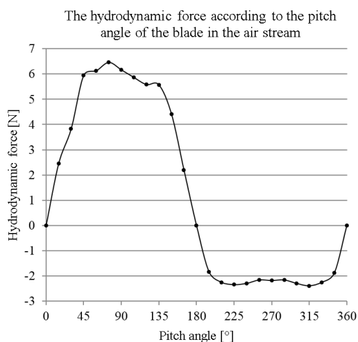
Fig. 8. The hydrodynamic force in dependence to the pitch angle of the single blade in the air velocity v = 14 m/s
