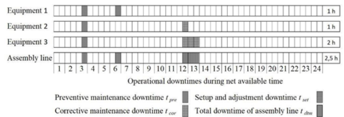
Fig. 3. Production line – downtime breakdown
