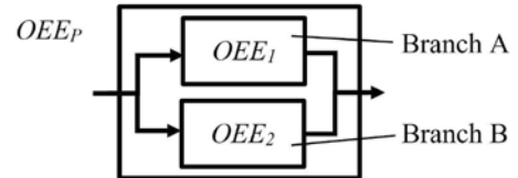
Fig. 5. Production line represented parallel system
