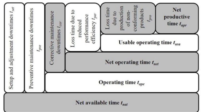
Fig. 1. Net available time breakdown [2]
