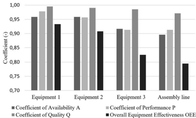
Fig. 4. Results of OEE calculation for serial system
