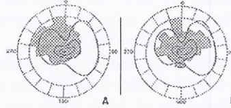
Figure 4: Three dimensional fishing boat noise directivity diagram according Misund (1987); A and B characterised the three-dimensional radiated noise change during fishing operation.
