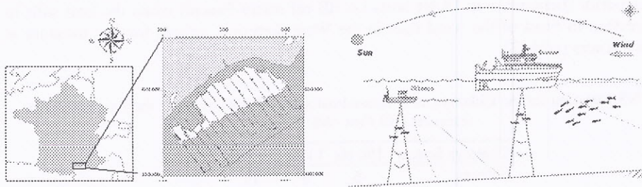
Figure 1: Map of the transects covered by the two boat during two days (29 July and 1 st August), area of common transect in white. The two boats used as in situ platform to record simultaneously the fish echo sounder data. The noise level emitted by the boat and its shadow, as stimulus on the fish behaviour, influence the sampling.
