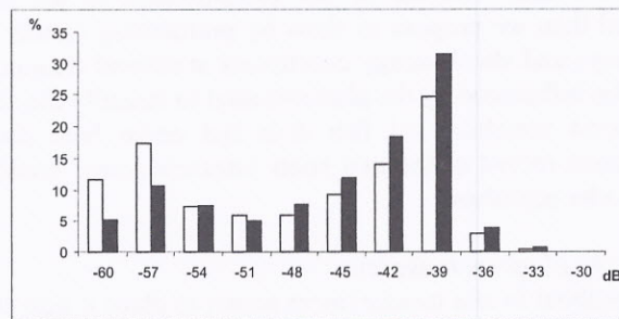
Figure 3: example of TS distributions from the EY500, 70 kHz (white) and EK500, 38 kHz (black), from the same area.
