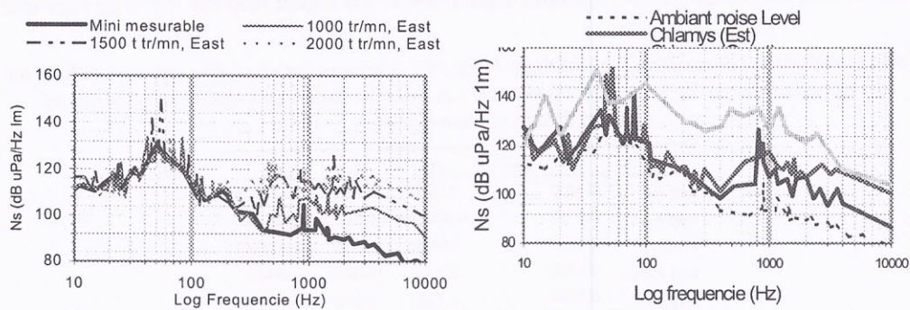
Figure 2: Noise in dB uPa/Hz 1 meters from 10 Hz to 10 kHz (logarithmic scale), generated by the Chlamys according to the bearing relatively to the wind direction (East blow). And the second spectral analysis compares the noise of the two boats at 8 knots and the ambient noise of the experiment area.
