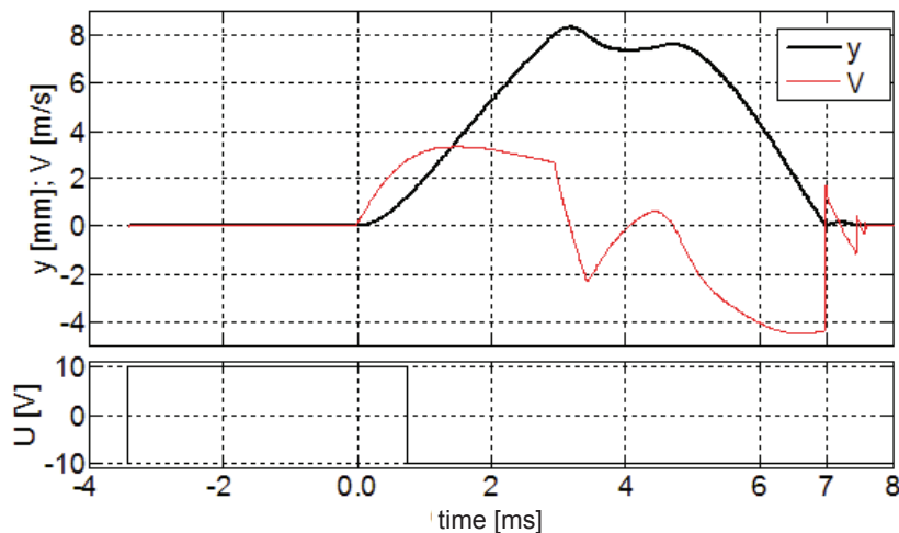
Fig. 7. Close to the theoretical waveforms of: valve lift, valve speed and the control signal for a supply pressure of 10 MPa and engine speed 6000 rpm without valve braking
