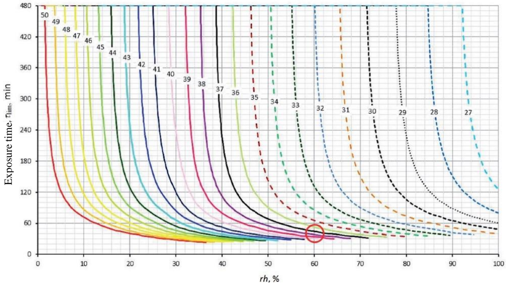
Fig. 1. Diagram for reading the allowed exposure time ( \tau_{im} ) of an employee wearing clothing with thermal insulation I_{cl} = 1 clo, staying in an environment with a temperature varying from 27^{\circ}\text{C} \leq t_a = t_r \leq 50^{\circ}\text{C} and relative air humidity in the range of 0\% \leq rh \leq 100\% , for energy expenditure M = 150 \text{ W/m}^2 (source: Sobolewski, 2014)
