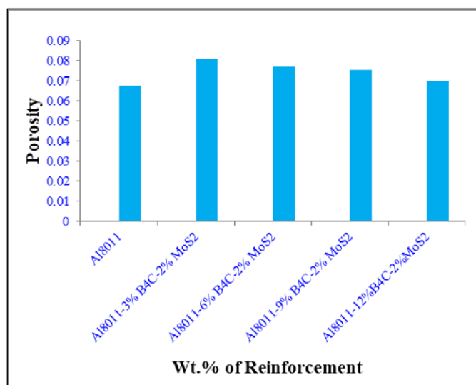
Fig. 9. Porosity in the Al8011- B_4C - MoS_2 composites
