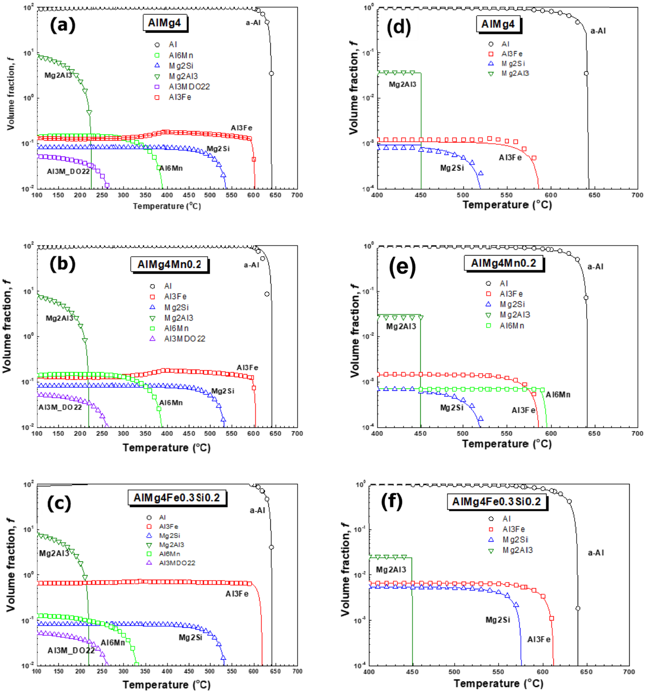
Fig. 1. Fraction solid of AIMg 4 , AIMg 4 Mn 0.2 and AIMg 4 Fe 0.3 Si 0.2 alloys calculated by J Mat Pro software: (a)-(c) equilibrium condition and (d)-(f) non-equilibrium condition
