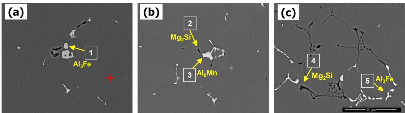
Fig. 2. Scanning electron micrographs of the samples homogenized at 500 ^{\circ}\text{C} for 24 h: (a) AIMg 4 , (b) AIMg 4 Mn 0.2 and (c) AIMg 4 Fe 0.3 Si 0.2 alloy
