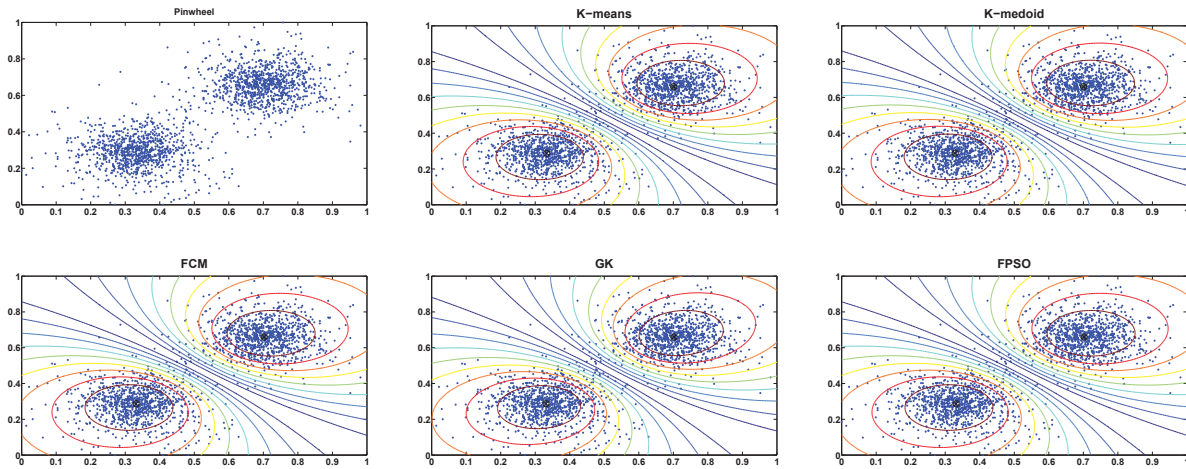
Figure 1: Synthetic data set
