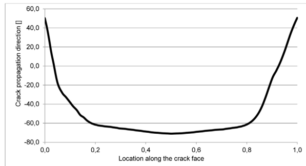
Fig. 10. The propagation direction of a ring crack ( \text{Si}_3\text{N}_4/\text{steel} combination, \gamma/\gamma_0 = -1.5 , friction coefficient between gap surfaces of 0.1)
