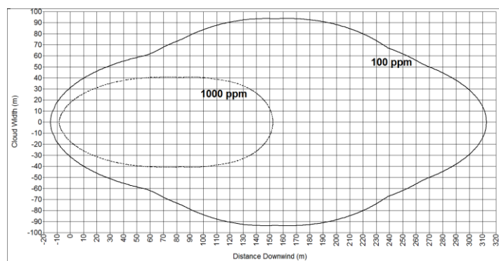
Fig. 2. Hazard zone due to an instantaneous release of chlorine ( u_w = 5 \text{ m/s} )
