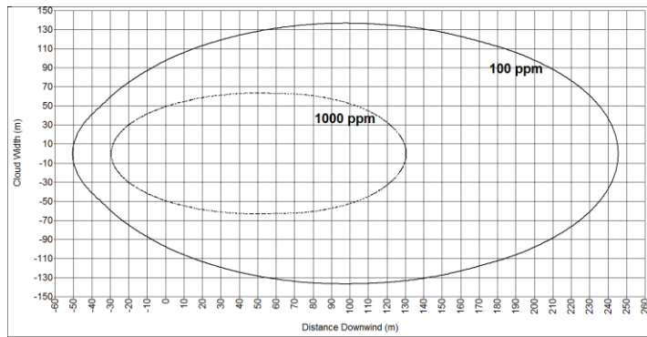
Fig. 1. Hazard zone due to an instantaneous release of chlorine ( u_w = 1.5 \text{ m/s} )
