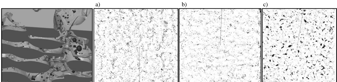
Fig. 6. CT visualization of air trapped in the ceramic coating a) A; b) Z and c) commercial
