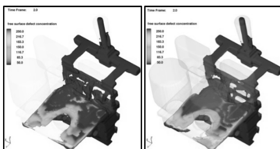
Fig. 9. Visualization of surface defect concentration a) gating system with applied filter; b) gating system without filter
