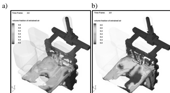
Fig. 8. Visualization of air closed by flowing liquid alloy a) gating system with applied filter; b) gating system without filter
