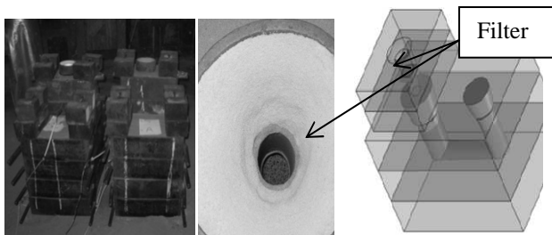
Fig. 2. Prepared molds for pouring trials, CAD model with marked filter nest
