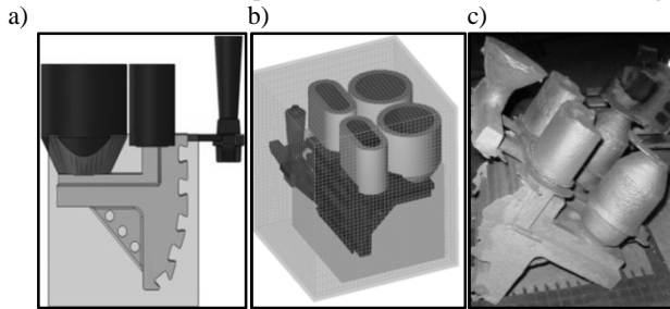
Fig. 7. a) CAD model with gating and risering system; b) workspace of simulation software; c) casting
