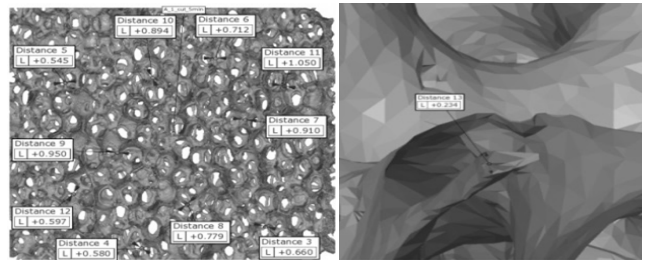
Fig. 4. The specified thickness of selected branch of foam filter A and the remains of the polyurethane skeleton
