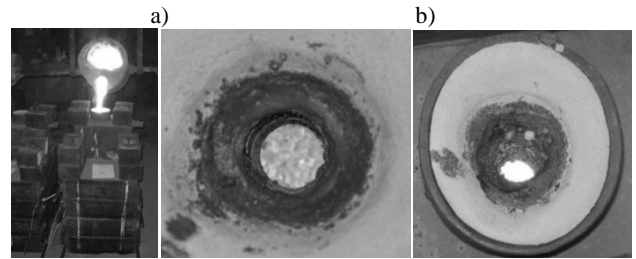
Fig. 3. Pouring trials, a) mold with filter, b) damaged filter
