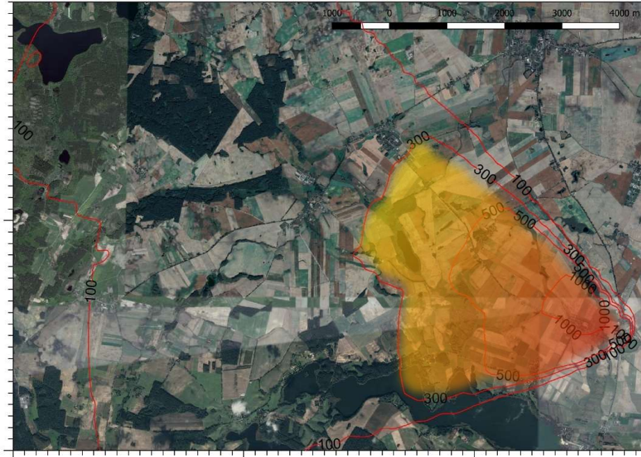
Fig. 2. Isolines of maximum concentrations of dust PM10, modelled for a fire in the period 28-29.05.2018 (variant I - emitter height: 1.5 m)
