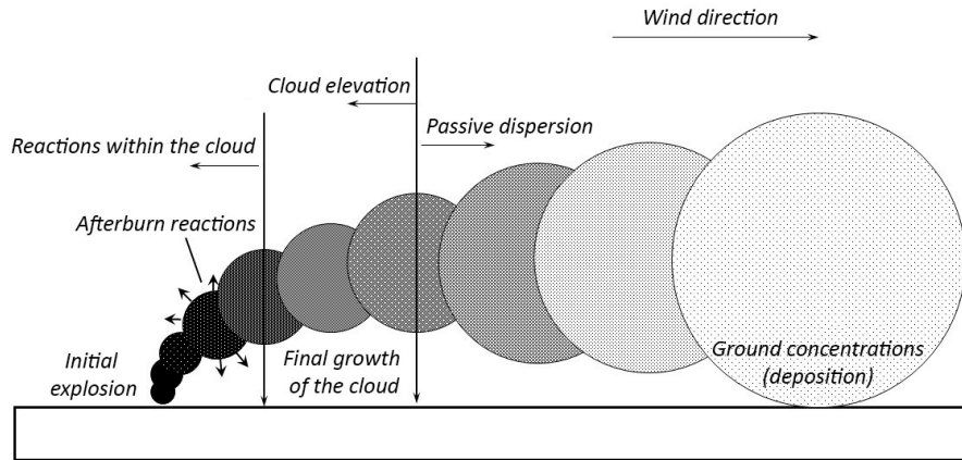
Fig. 1. Spreading of the pollution cloud based on the assumptions of the Source Characterisation Model (SCM), based on [Brown et al., 2004]
