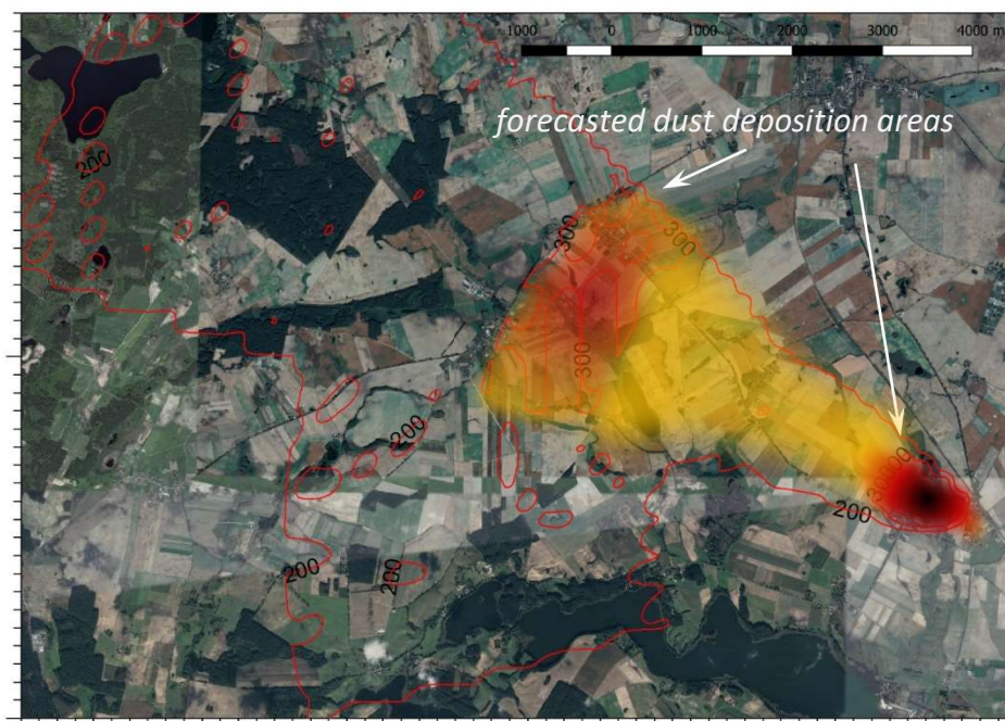
Fig. 3. Isolines of maximum concentrations of dust PM10, modelled for the fire on 28-29.05.2018 (variant II - emitter height: 60 m)
