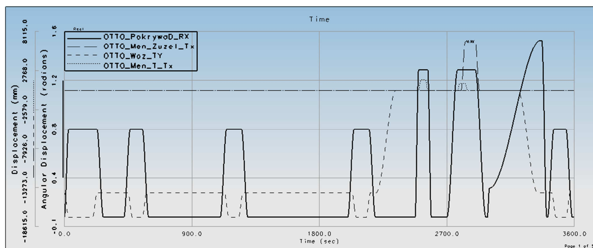
Fig. 3. Motion diagram
