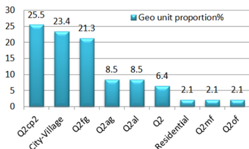
Fig. 10. The proportion of geo units around the wells; source: own study
