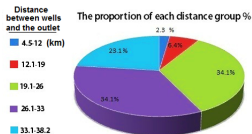
Fig. 12. Distances of the wells up to the outlet; source: own study
