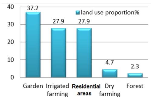
Fig. 8. The proportion of land use types around the wells; source: own study
