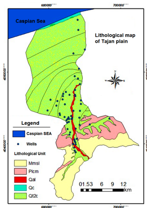
Fig. 11. The lithological map of the Tajan Plain; source: own elaboration
