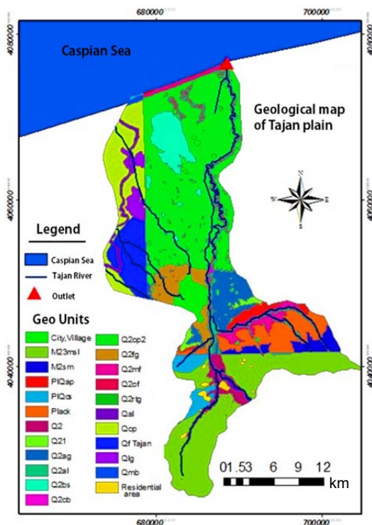
Fig. 9. The geological map of the Tajan Plain; source: own elaboration
