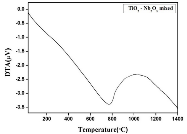
Fig. 4. DTA plot of the \text{TiO}_2 - \text{Nb}_2\text{O}_5 mixed powder heated at a rate of 1^\circ\text{C}/\text{min}
