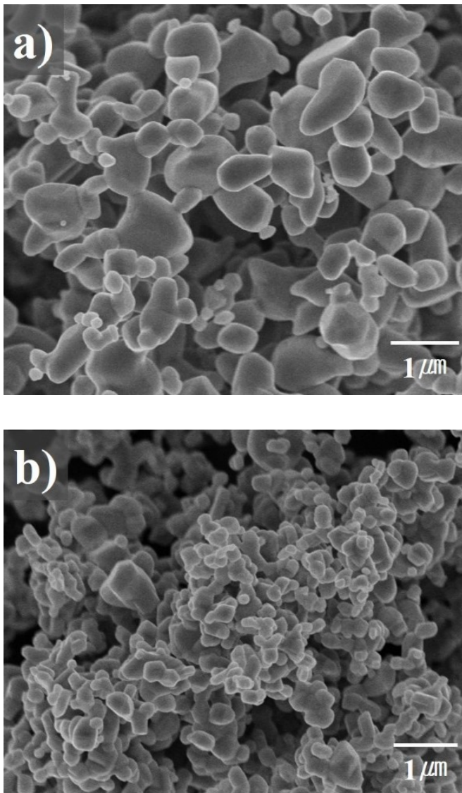
Fig. 3. SEM morphologies of the starting materials; a) \text{TiO}_2 powder and b) \text{Nb}_2\text{O}_5 powder
