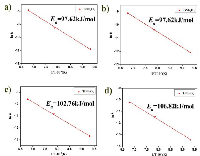
Fig. 10. Arrhenius plots for samples synthesized at temperatures in the range of 800-1200°C for a) 1 h, b) 5 h, c) 10 h, and d) 20 h
