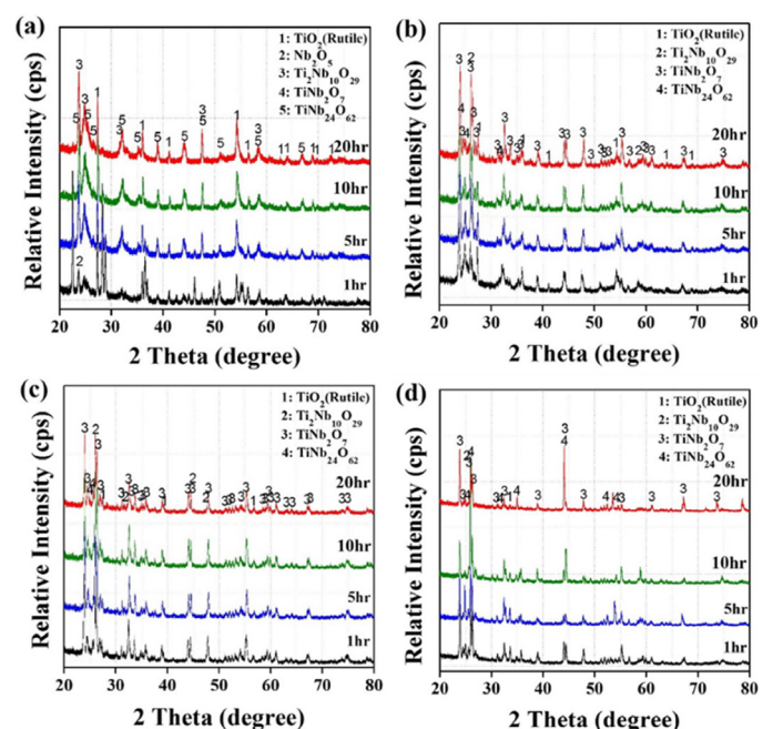
Fig. 5. XRD patterns of the Ti-Nb-O samples heat-treated at (a) 800^\circ\text{C} , (b) 1000^\circ\text{C} , (c) 1200^\circ\text{C} , and (d) 1400^\circ\text{C}
