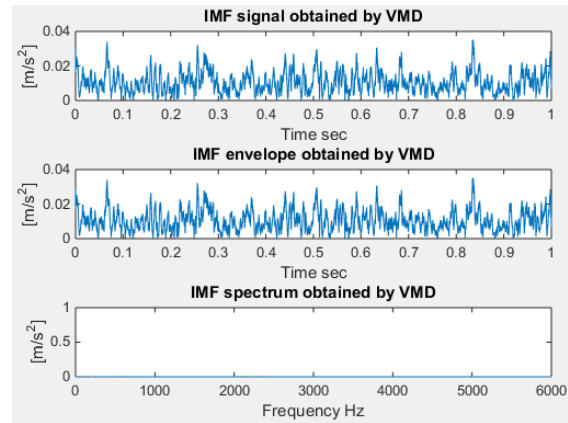
Fig. 5. Optimal IMF of VMD
